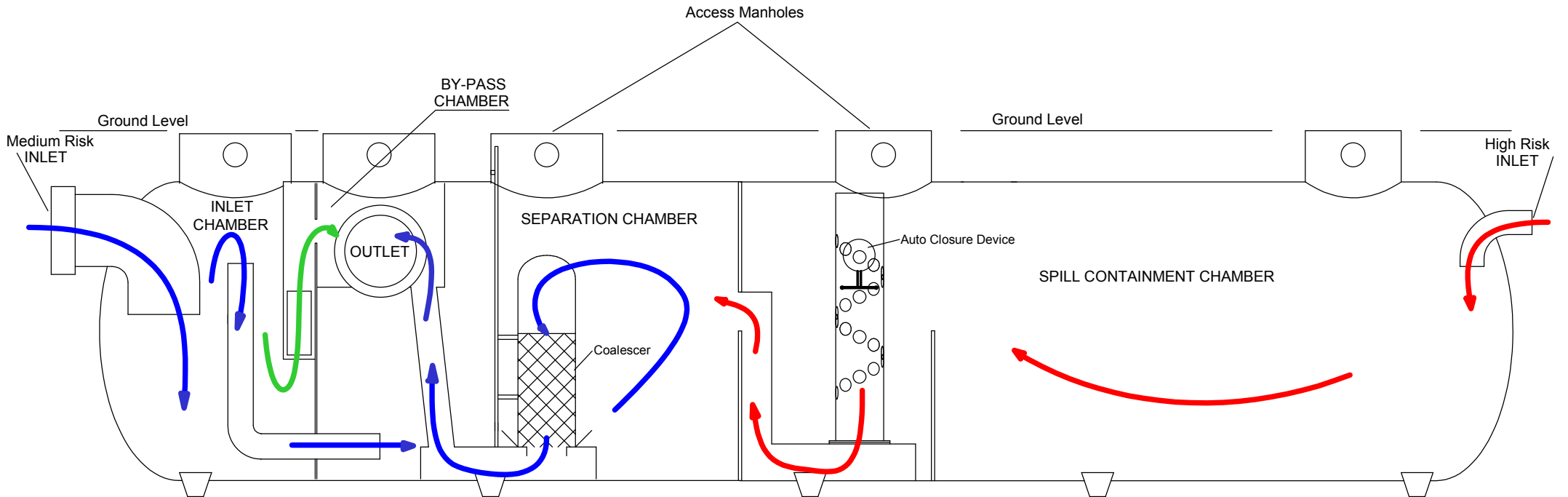
Sectional Side View.
