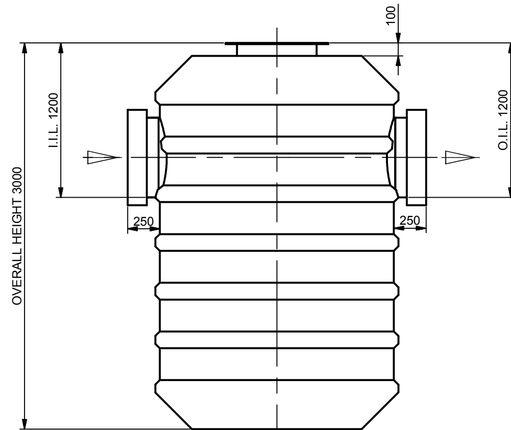
ELEVATION VIEW
