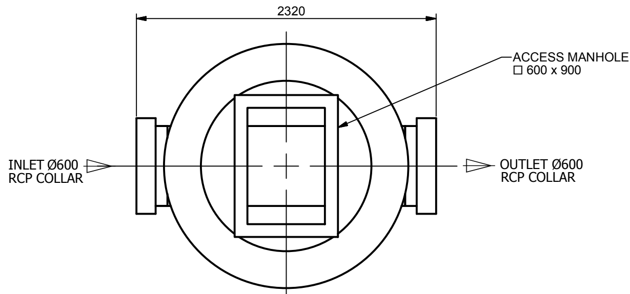
PLAN VIEW
